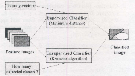
Figure 4: Supervised and unsupervised classification
