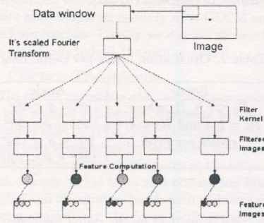
Figure 3: Flow diagram for feature image formation
